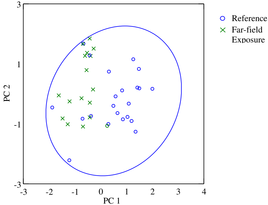
Figure 4 An example of the graphical presentation of fish tissue chemistry data using PCA.
