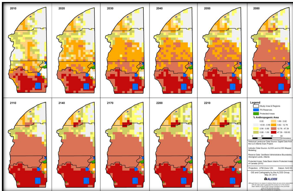
Figure 155. Simulated future change in land-use footprint area (%) in CLFN SA if reclamation rates are set at 0.
