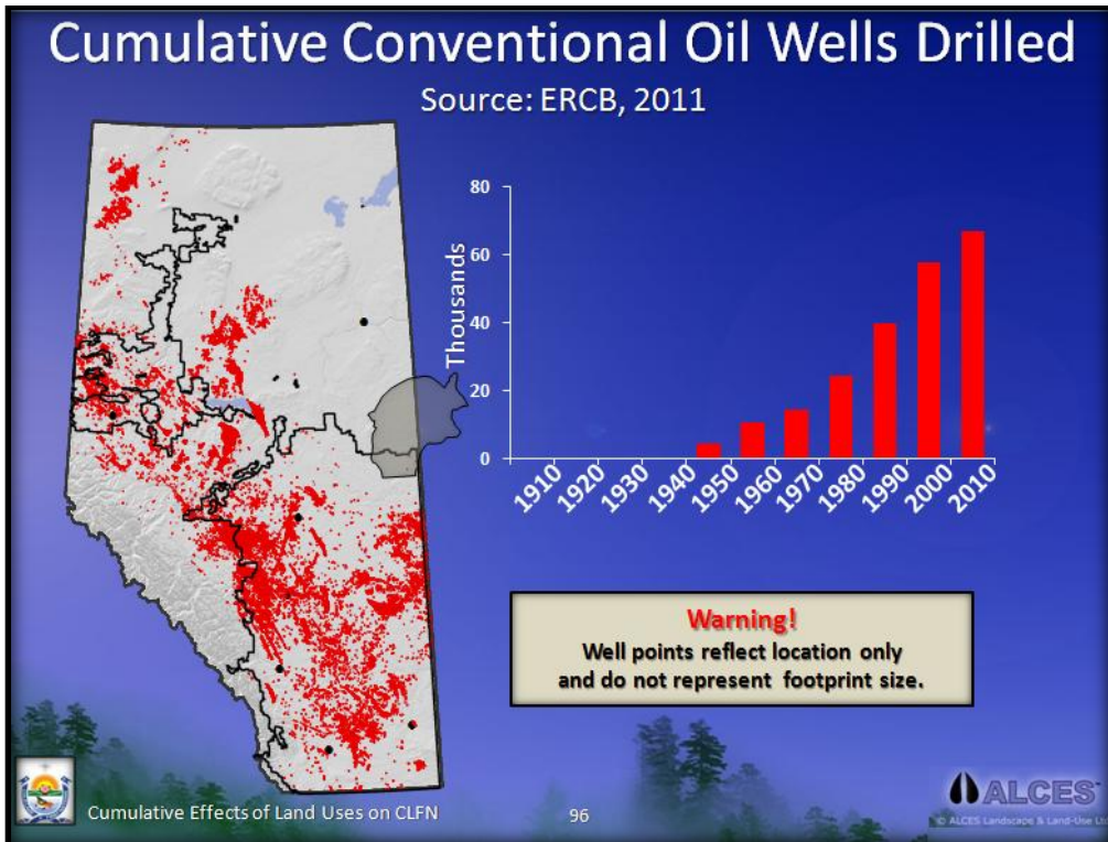
Figure 76. CLFN SA in context of historical conventional oil production in Alberta. Source: ERCB, 2011.
