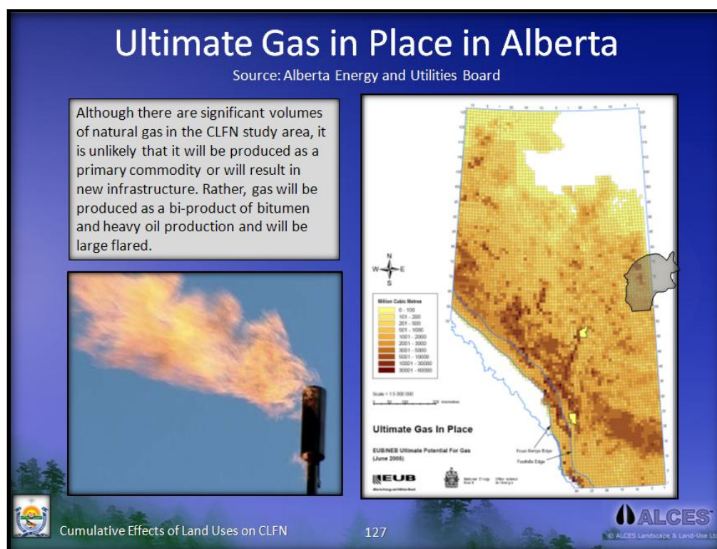
Figure 83. Ultimate Gas in Place in Alberta and in relation to the CLFN SA. Source: Alberta Energy and Utilities Board.
