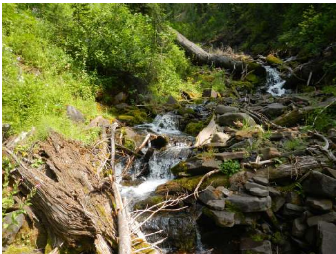
Figure 6. Step-pool channel in Alexander Creek (credit: J. Smithson).
