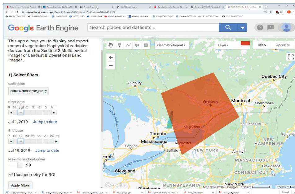
Figure 3.1 – Landscape Evolution and Forecasting (LEAF) Toolbox running Version 0 algorithm.
