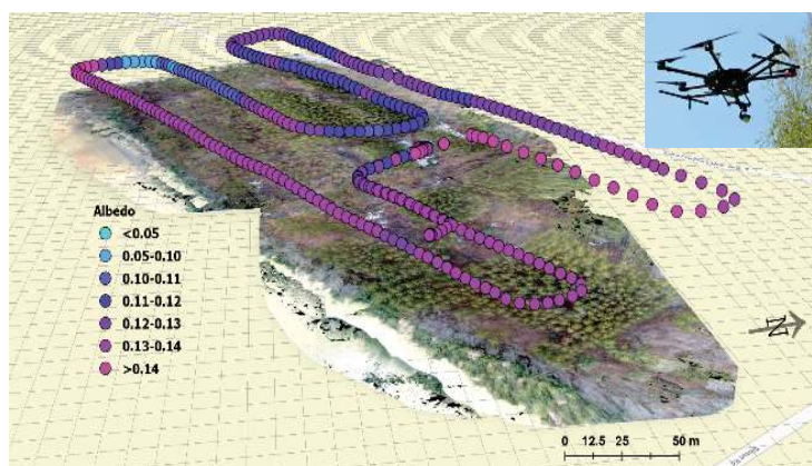
Figure 11.1 – Pyranometer sensor measured albedo (preliminary results) overlaid on a visible orthomosaic at Turkey Point in southern Ontario. Data from sensors mounted on a M600 UAV.
