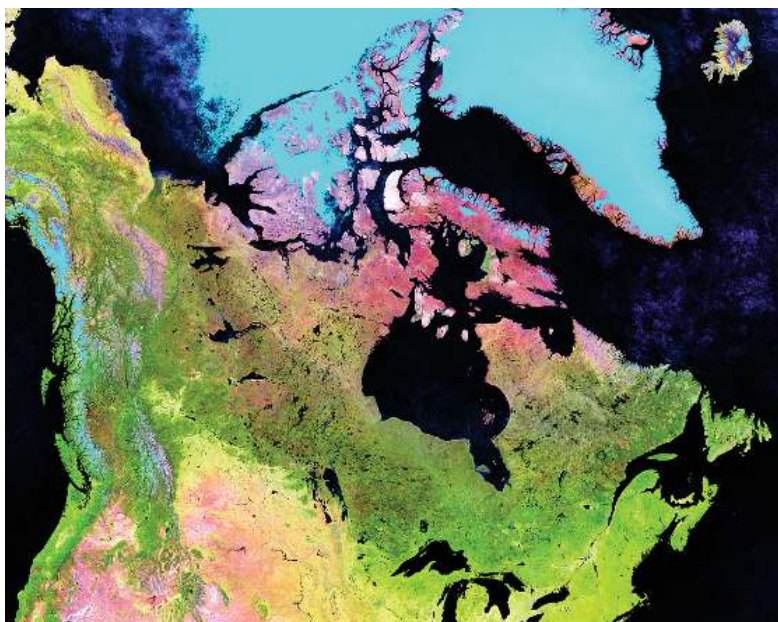
Figure 7.1 – False color warm season (April – September) clear-sky composite over Canadian landmass corresponding to minimum snow/ice cover for 2019 at 250-m spatial resolution. MODIS/Terra.
