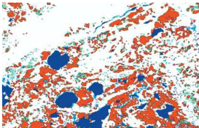
Figure 4.3 – Discontinuous permafrost (pink) in the Lidar image (left) is well identified in the radar image (orange). The results show that the long penetrating radar is promising to detect and map permafrost accurately.
